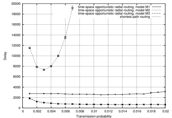
Fig. 8. Comparison between routing strategies: end-to-end delay versus transmission probability p .
