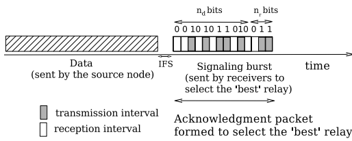
Fig. 3. Structure of the acknowledgment packet to select the 'best' relay towards the destination.
