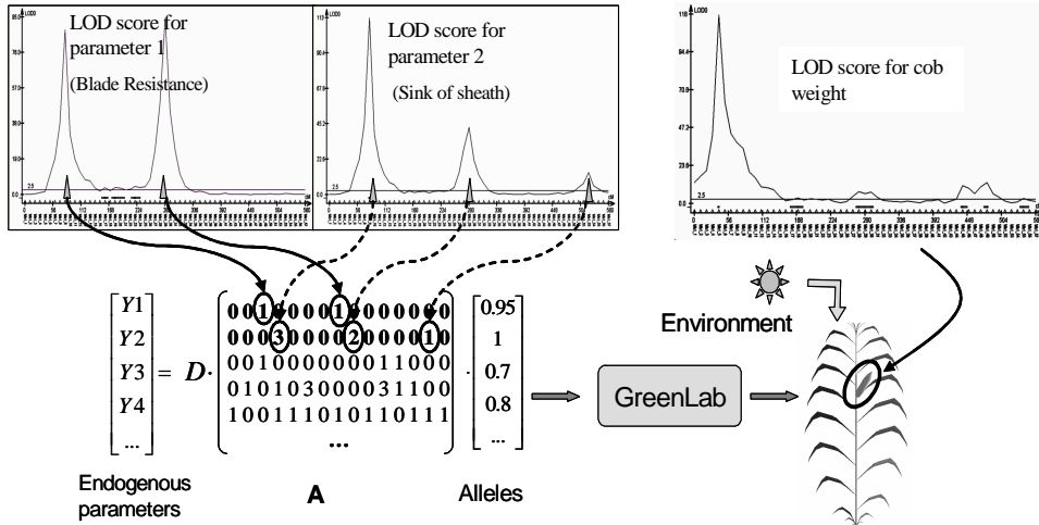
Fig. 5. Simulation of QTL detection: GreenLab parameters ( Y ) are determined through a simple genetic model (matrix multiplication D, A ) from the allele values. The graphs represent the results of QTL detection using a virtual mapping population when traits are model parameter compared to the case where the trait is cob weight.
