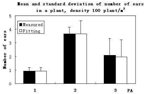
Fig.2. The mean and standard deviation of the number of phytomers and ears in main stem (PA 1), primary tillers (PA 2), secondary tillers (PA 3) of a wheat plant, with population density 100 plants m -2 , fitted with GreenLab organogenesis model (lines).
