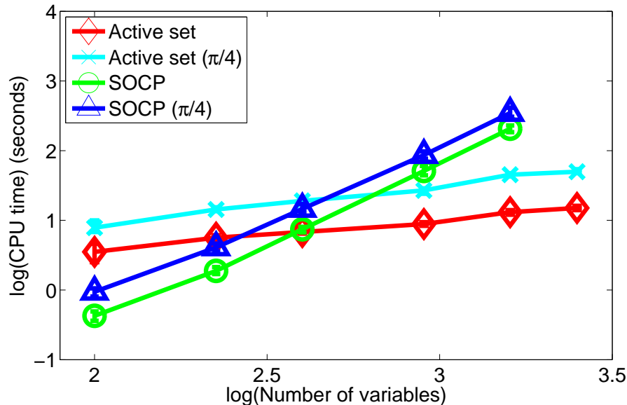
Figure 12: Computational benefit of the active set algorithm: CPU time (in seconds) versus the number of variables p , displayed in log-log scale. The points, the lower and upper error bars on the curves respectively represent the median, the first and third quartile. Two sets of groups \mathcal{G} are considered, the rectangular groups with or without the \pm\pi/4 -groups (denoted by (\pi/4) in the legend). Due to the computational burden, we could not obtain the SOCP's results for p = 2500 .
