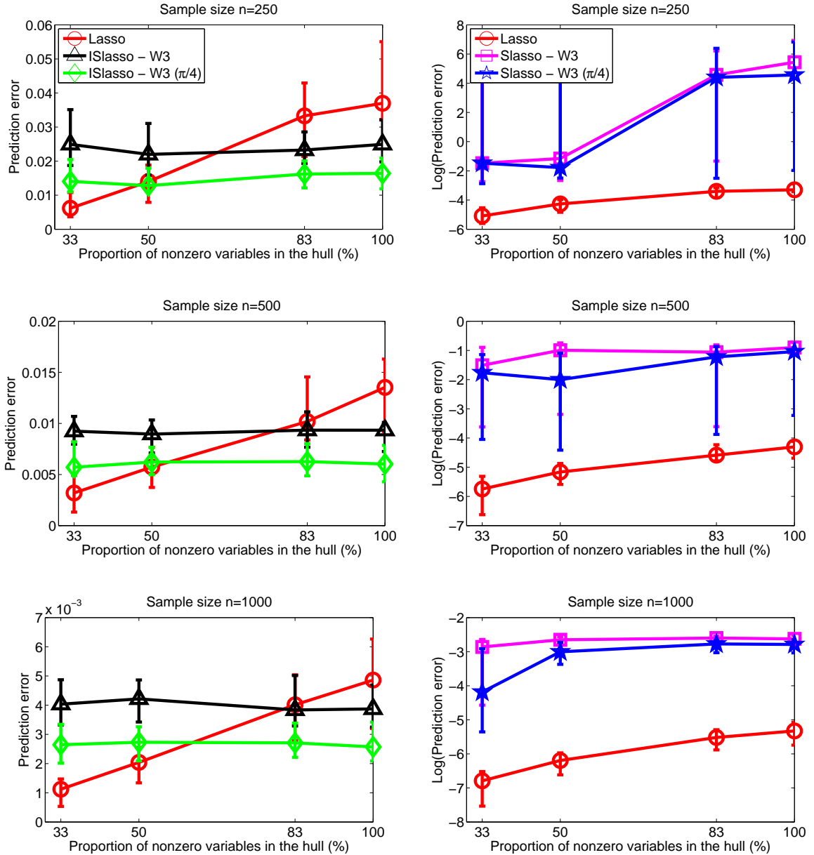
Figure 11: Experiments on the grid: for the sample sizes n \in \{250, 500, 1000\} , we plot the prediction error versus the proportion of nonzero variables in the hull of the generating pattern. We display the results on two different columns since the models obtain very heterogeneous performances (on the right column, the error is in log scale). The points, the lower and upper error bars on the curves respectively represent the median, the first and third quartile, based on 50 random settings \{\mathbf{J}, \mathbf{w}, X, \varepsilon\} . Two sets of groups \mathcal{G} are considered, the rectangular groups with or without the \pm\pi/4 -groups (denoted by (\pi/4) in the legend). In addition, we have dropped for clarity the models that performed poorly on the sequence.
