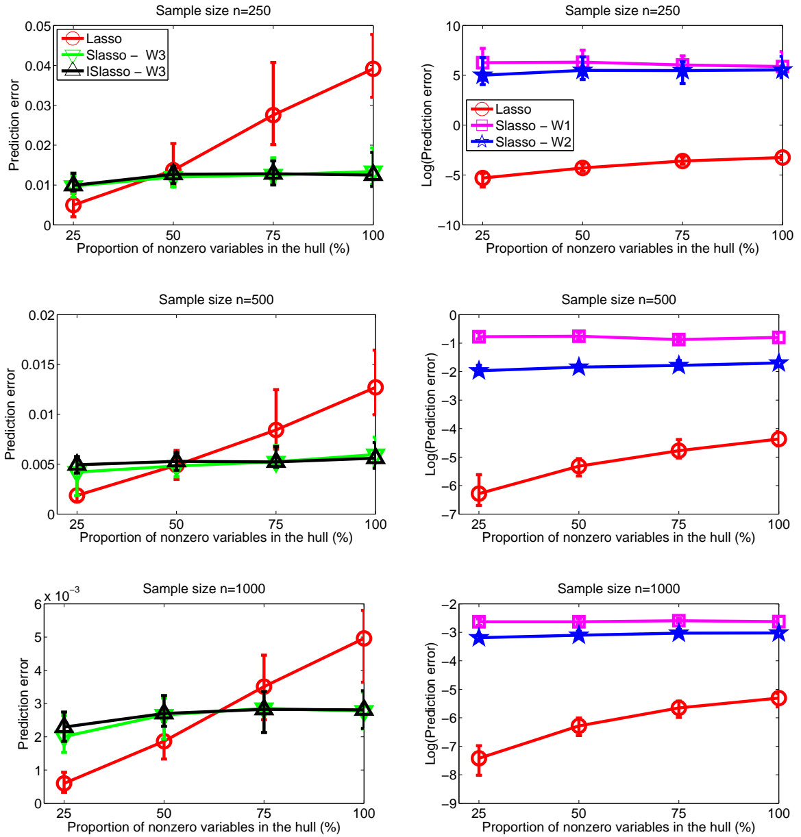
Figure 10: Experiments on the sequence: for the sample sizes n \in \{250, 500, 1000\} , we plot the prediction error versus the proportion of nonzero variables in the hull of the generating pattern. We display the results on two different columns since the models obtain very heterogeneous performances (on the right column, the error is in log scale). The points, the lower and upper error bars on the curves respectively represent the median, the first and third quartile, based on 50 random settings \{\mathbf{J}, \mathbf{w}, X, \varepsilon\} .
