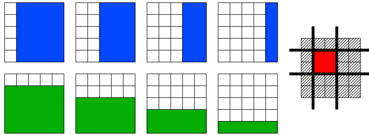
Figure 5: Vertical and horizontal groups: (Left) the set of blue and green groups with their (not displayed) complements to penalize in order to select rectangles. (Right) In red, an example of recovered pattern in this setting.
