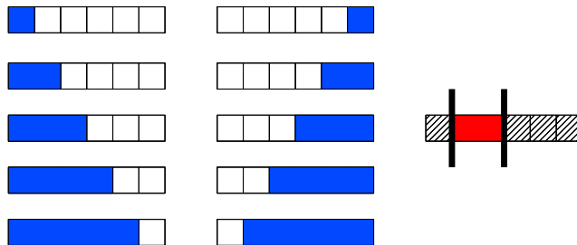
Figure 4: (Left) The set of blue groups to penalize in order to select contiguous patterns in a sequence. (Right) In red, an example of such a pattern.
