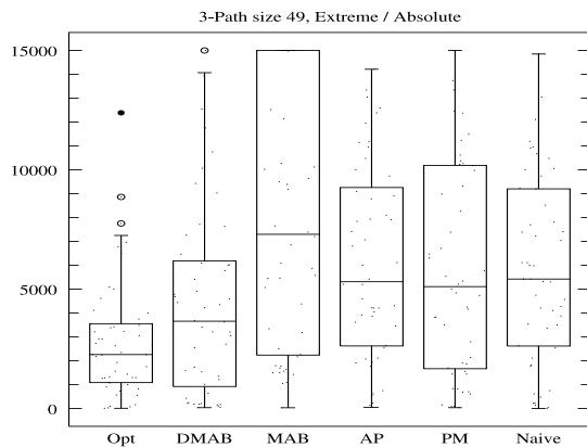
Figure 2: AOS performances on Long K -Path, using the Extreme/Absolute Credit Assignment . From left to right: optimal strategy, Dynamic Multi-Armed Bandit, Multi-Armed Bandit, AP, PM and the naive uniform strategy.
