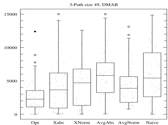
Figure 3: AOS performances on Long K -Path, using the Dynamic Multi-Armed Bandit Operator Selection . From left to right: optimal strategy, ExtremeAbsolute, ExtremeNormalized, AverageAbsolute and AverageNormalized Credit Assignment , and the naive uniform strategy.
