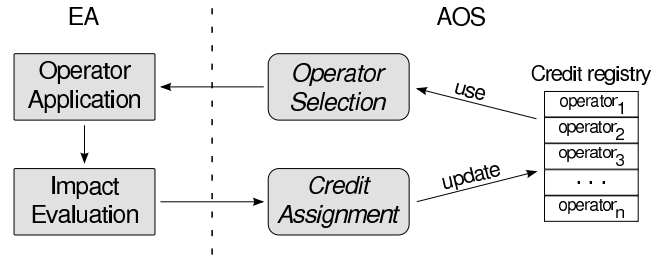
Figure 1: The Adaptive Operator Selection scheme.
