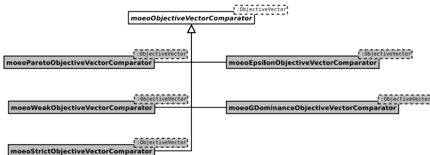
Figure 6: UML diagram for dominance relation (used for pairwise objective vector comparison).
