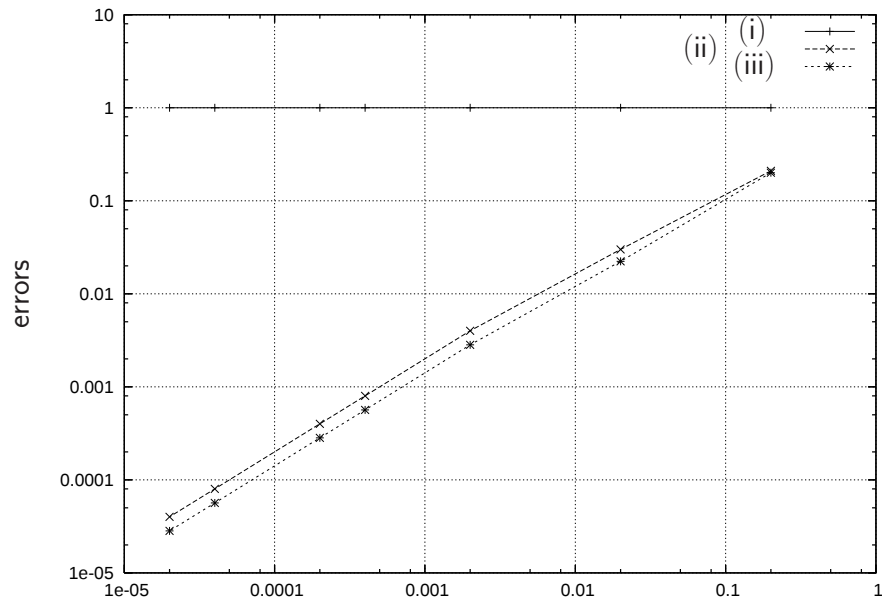
(d) Numerical error \|e_s\|_\infty (solid line (i)), \|e_s\|_1 (dashed line (ii)), \|e_s\|_2 (dotted line (iii)), with respect to h in logscale
