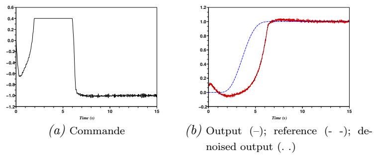
Figure 9. Unstable nonlinear system: saturated control with anti-windup
