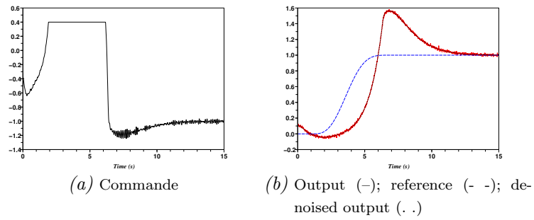
Figure 8. Unstable nonlinear system: saturated control without anti-windup
