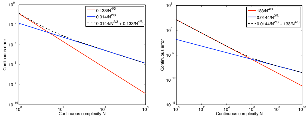
Figure 10: Left, convergence history obtained for the function u_3 on the set of inhomogeneous continuous meshes spans by \mathbf{I}(\alpha) defined on \Omega_2 . Right, convergence history for the error function of Remark 4. In that case, the coefficients involved in the error expression lead to observe O(N^{-\frac{4}{3}}) as predominant term in the reachable range of complexity [1, 10^6] whereas the asymptotic convergence order is O(N^{-\frac{2}{3}}) .
