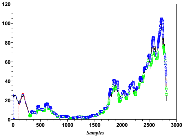
Figure 6. Prices (black, -), filtered signal (blue, .), 5 day forecast (red, - -), forecast of the prices above the predicted trend (green \Delta ), forecast of the prices below the predicted trend (blue \nabla ) (5 days)
