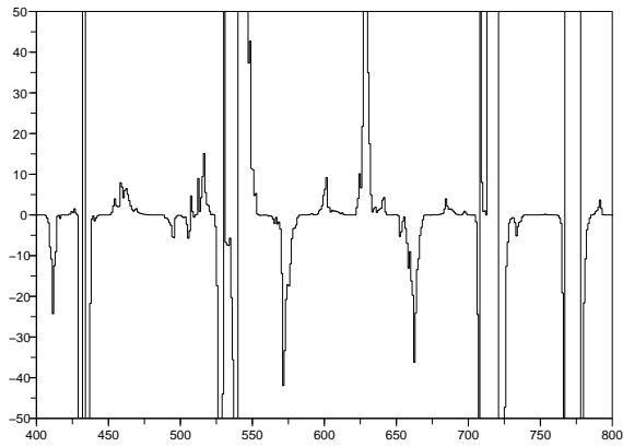
Figure 9. SKEW_5 (5 days)
