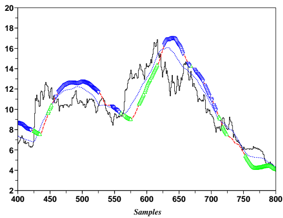
Figure 11. Zoom of Figure 10 (10 days)
