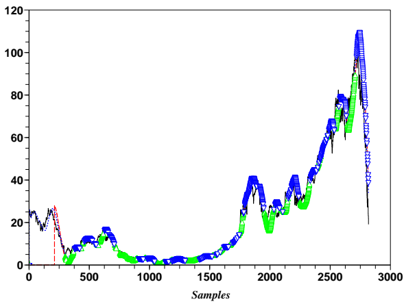
Figure 10. Prices (black,-), filtered signal (blue,.), 10 day forecast (red, - -), price's forecast higher than the predicted trend (green \Delta ), price's forecast lower than the predicted trend (blue \nabla ) (10 days)
