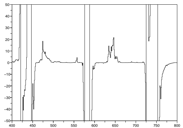
Figure 13. SKEW_{10} (10 days)
