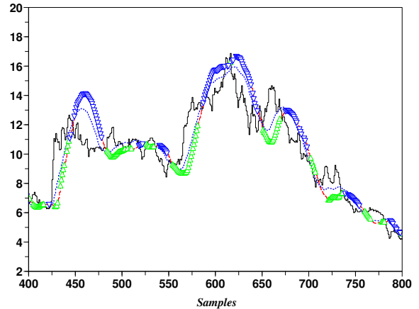
(a) Zoom of 6
