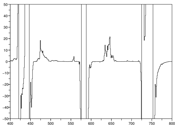
Figure 13. SKEW_{10} (10 days)
