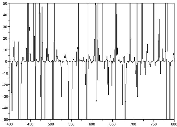
Figure 5. SKEW 1 (1 day)
