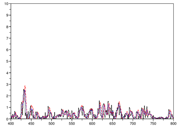
Figure 4. ABS-DIFF 1 (black,-), filtered signal (blue,.), 1 day forecast (red, - -) (1 day)
