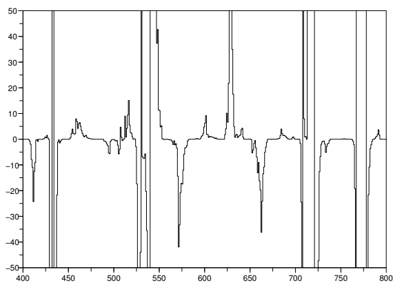
Figure 9. SKEW_5 (5 days)
