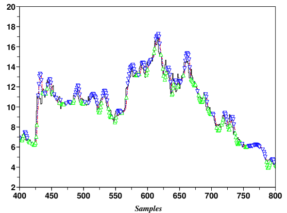
Figure 3. Zoom of Figure 2 (1 day)
