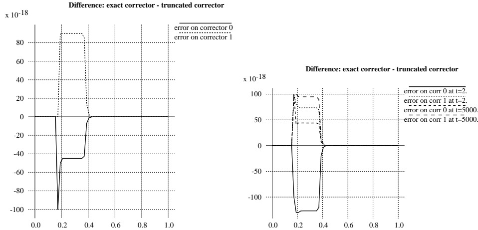
FIG. 3.1. Difference between the correctors for f(t, x) = x (on the left) and f(t, x) = x + \sin(t) (on the right), for \varepsilon = 0.01 and a time step equal to 0.1 . We define the boundary layer length as 0.1 , and consider 31 points in the boundary layer, 51 points outside.
