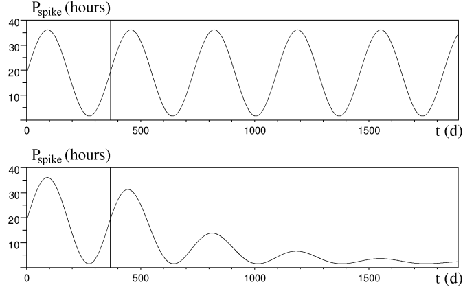
FIGURE 4. Graphs of the two functions used successively for P_{spike} . The top panel represents the sinusoid function defined by (2.5); the second one is defined by (2.6) as the same sinusoid over [0, 1 \text{ year}] , and, over [1 \text{ year}, 5 \text{ years}] , a damped sinusoid with same fundamental period and damping coefficient \zeta = 0.14 . The vertical segment at 1 year represents the beginning of the sampling process on the fine numerical integration of equation (2.8).
