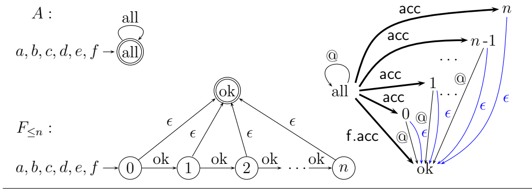
Figure 16: Example run of the algorithm: \text{f.frb}_1^c(\text{all}, \{0, \dots, n-1\}) is inferred.
