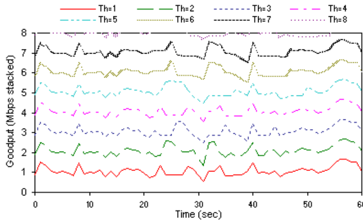
Figure 5: Goodput for different values of threshold
