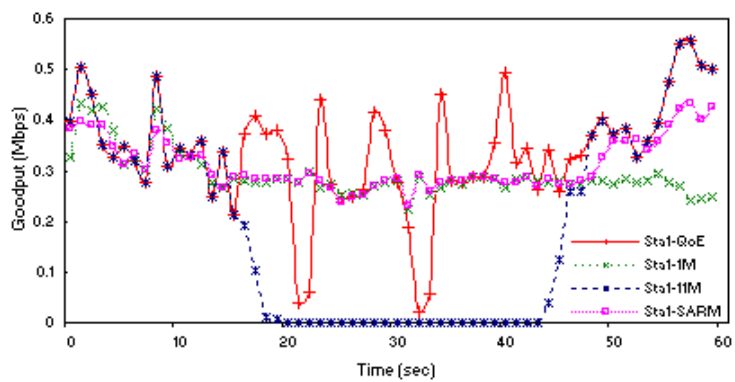
Figure 8: Goodput of a moving station
