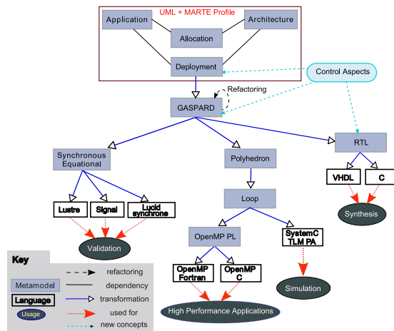
Figure 12: Gaspard framework with added concepts for integration of PDR aspects
