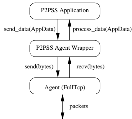
Figure 1: Simulator architecture.
