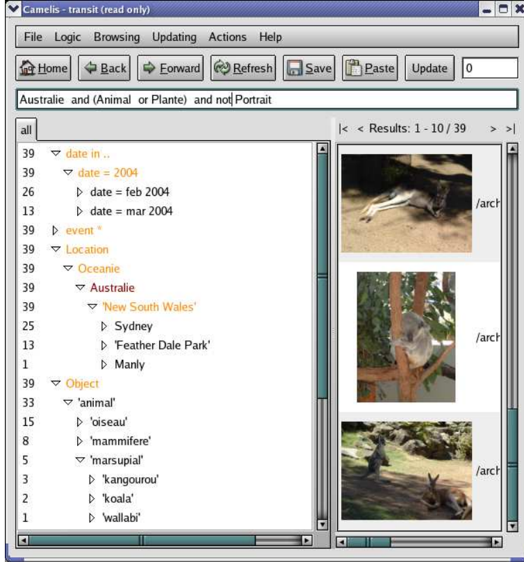
Figure1. A screenshot of the graphical interface of CAMELIS.
