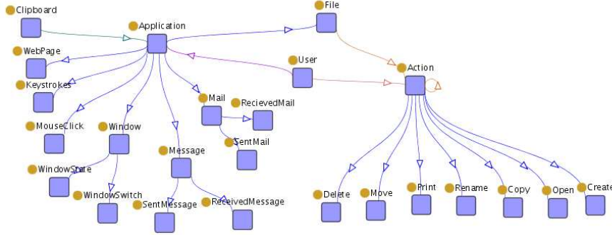
Figure 2: Trace Model Example
