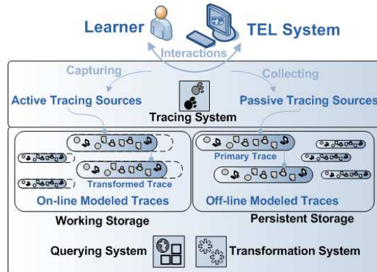
Figure 1: Trace-Based System Architecture
