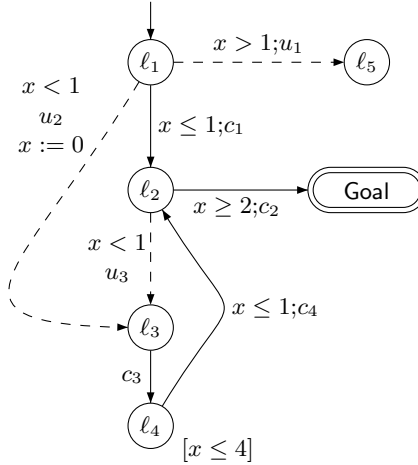
Fig. 1. A Timed Game Automaton
