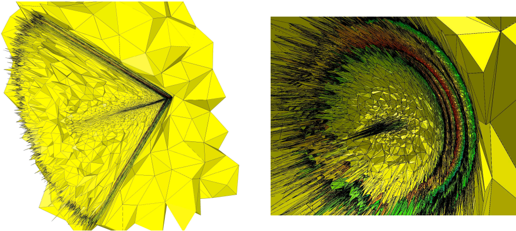
Figure 2: 3D supersonic aircraft simulation. Two views of the final anisotropic adapted mesh containing 3, 764, 591 vertices and 22, 324, 258 tetrahedra throughout cut planes. The global (left) and the close-up views point out the highly anisotropic feature of the mesh.
