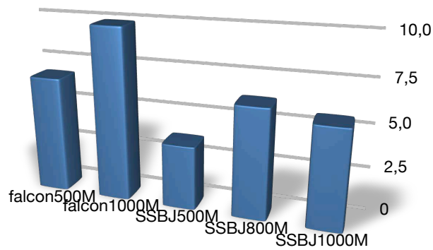
Figure 7: Speed-ups obtained for the adaptive mesh generator Mmg3d with the Hilbert renumbering for each test case of the benchmark data base. In each case, the renumbered version of the serial code is at least twice faster than the original serial code. These speed-ups include the reordering time.
