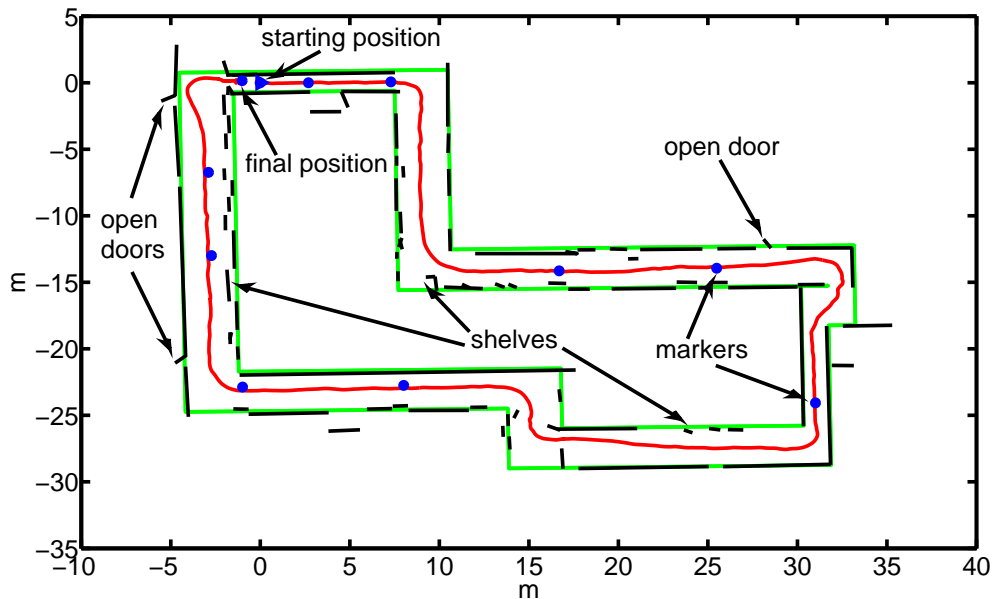
Fig. 5. Complete map of the Department corridors; 130m long trajectory. The unit of coordinate-axis is meter.
