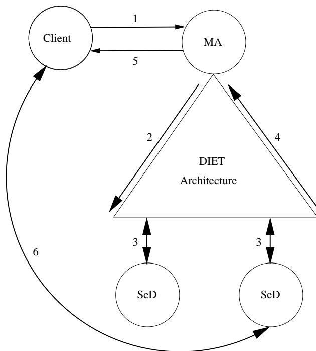
Figure 2: A DIET architecture.
