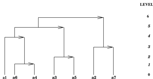
Figure 1: Tree associated with a binary directed hierarchy
