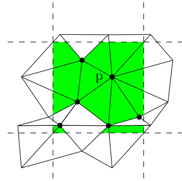
Figure 3: (2D case) The shaded region is \varphi_{\mathbf{c}}(\text{St}(p) \times \mathbb{Z}^3) \cap \mathcal{D}_{\mathbf{c}} . There are several cycles of length two originating from p .
