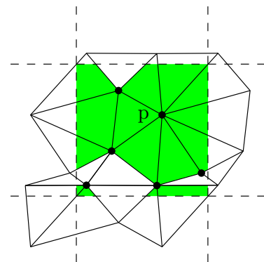
Figure 3: (2D case) The shaded region is \varphi_c(\text{St}(p) \times \mathbb{Z}^3) \cap \mathcal{D}_c . There are several cycles of length two originating from p .
