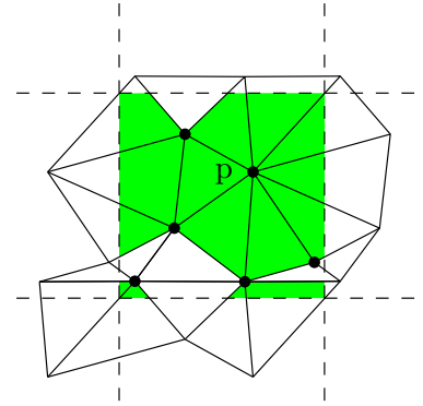
Figure 3: (2D case) The shaded region is \varphi_{\mathcal{C}}(\text{St}(p) \times \mathbb{Z}^3) \cap \mathcal{D}_{\mathcal{C}} . There are several cycles of length two originating from p .
