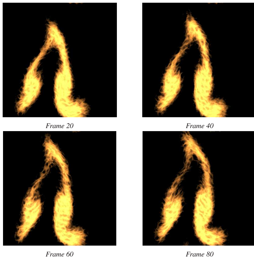
Figure 7: Apply advected noise to a fire shader.
