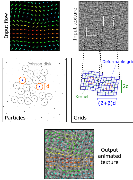
FIG. 1 – Overview of our algorithm. Top : we take as input an animated velocity field and a texture. Middle : we advect particles by the flow. We maintain a Poisson disk distribution, killing or creating new particles when necessary. A deformable grid is attached to each particle and mapped to a fixed area of the input texture. Bottom : we blend these deformable textured grids to get our animated texture.
