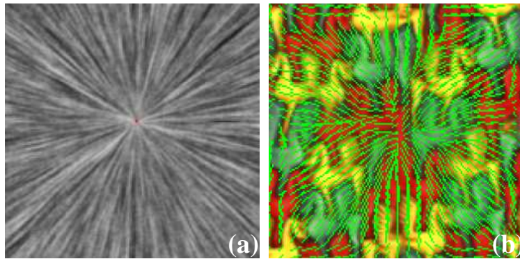
FIG. 5 – Comparison with animated texture synthesis. The optical flow (b) does not accurately match the input velocity field (a) (measured here on [Kawtra et al. 2005]).
