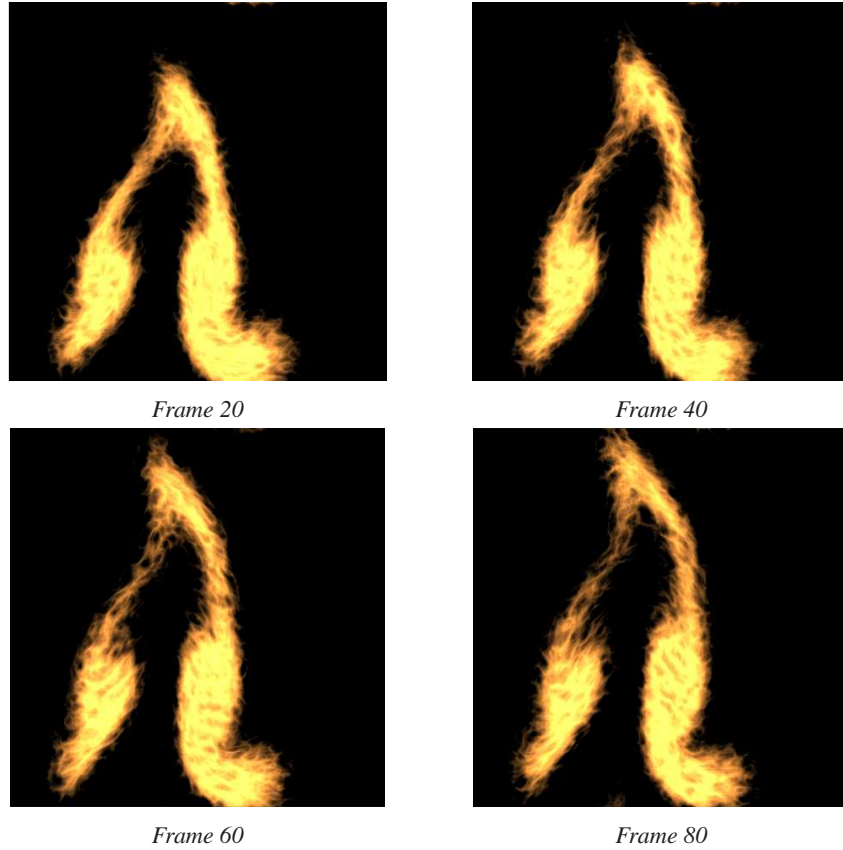
FIG. 7 – Apply advected noise to a fire shader.
