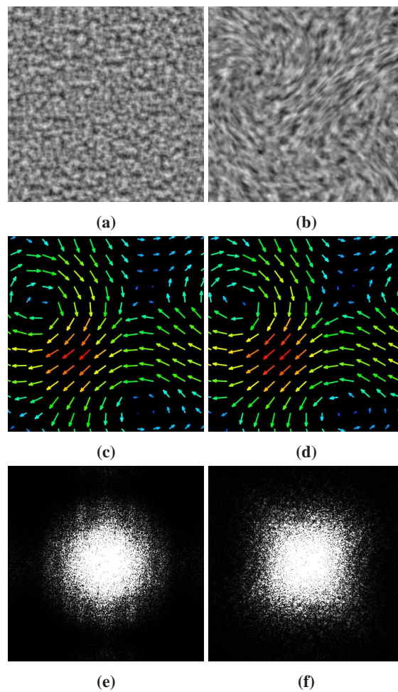
FIG. 3 – Quality of our generated animated textures. Left : input texture (a), input flow (c) and Fourier spectrum (e) of input texture. Right : our advected texture (b), its optical flow (d) and its Fourier spectrum (f).
