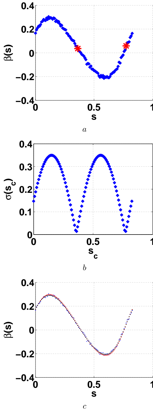
Figure 8: The estimation of the nodes and then the parameters \xi_q , L , c and k for q = 0.6 for the robot e-puck without tape. a displays the observation function with the estimated nodes, b displays the function \sigma(s_c) and c displays the observation function as observed (blue points), as estimated by our strategy alone (red points) and improved with the Levenberg Marquadt algorithm (black points).
