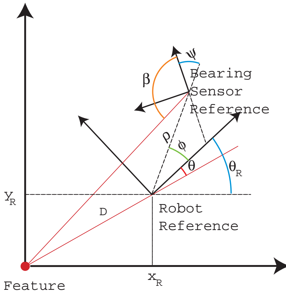
Figure 1: The two reference frames respectively attached to the robot and the bearing sensor.
