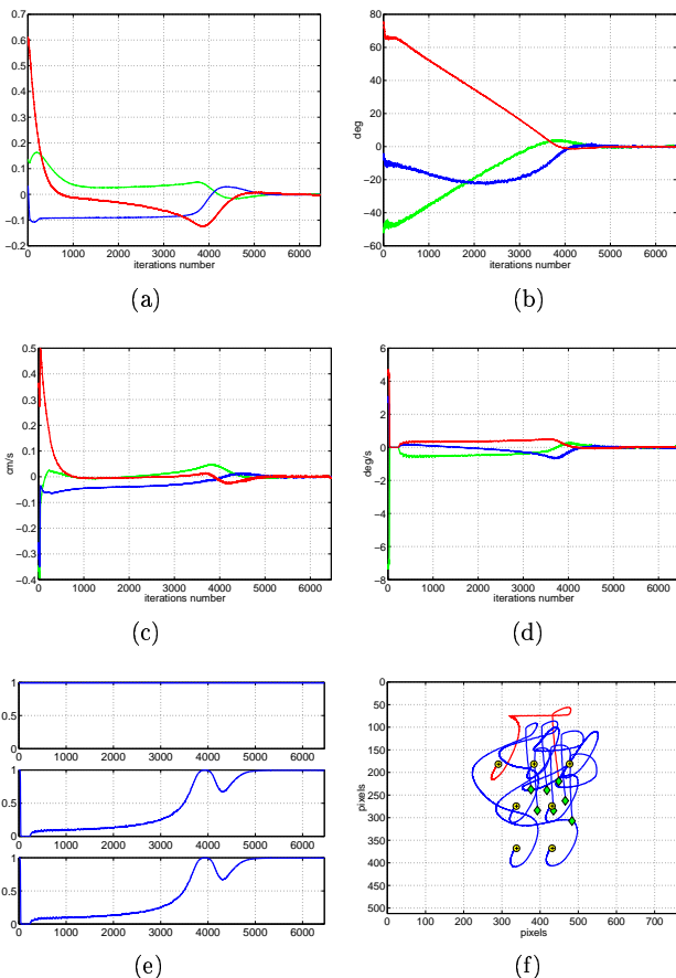
Fig. 17. Robust control law: (a) error in extended image coordinates, (b) rotation u\theta , (c) translational velocity, (d) rotational velocity, (e) gains f_u , f_v and f_u f_v , and (f) trajectories in the image of the target points.
