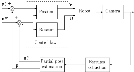
Fig. 4. Block diagram of the 2 1/2 D visual servoing.
