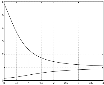
Fig. 7. Stability bounds for relative depth \hat{d}^*/d^* .
