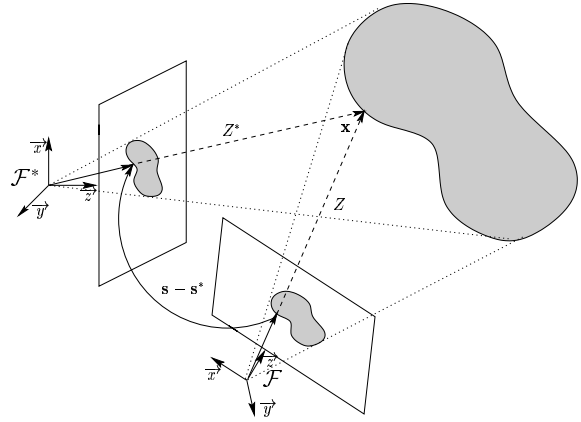
Fig. 2. 2D visual servoing.
