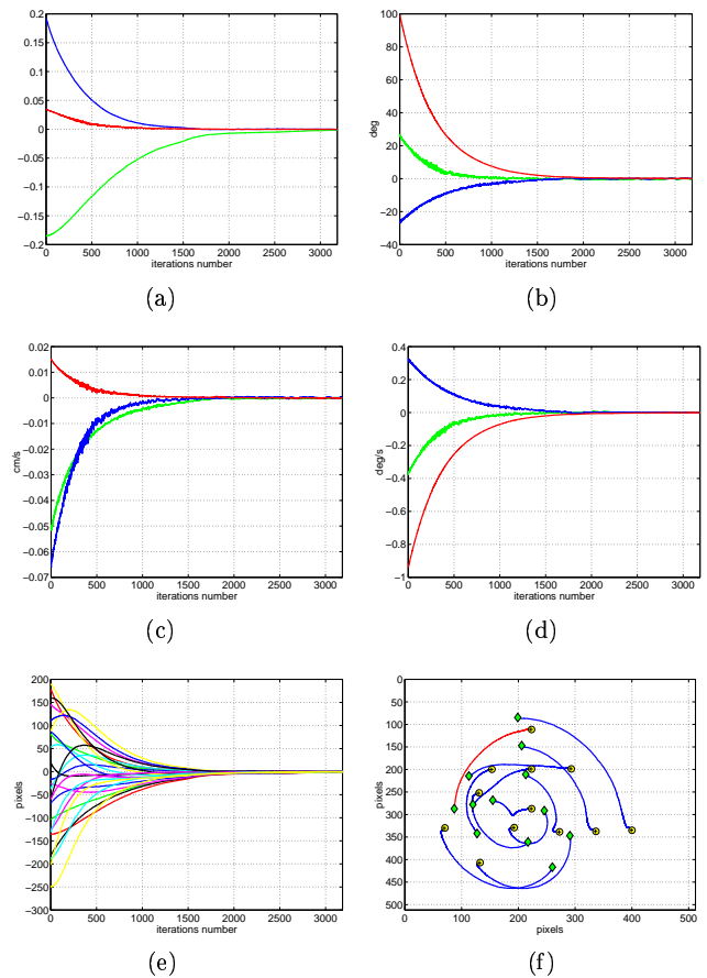
Fig. 13. Results of 2 1/2 D visual servoing with bad camera and hand-eye calibration: (a) error in extended image coordinates, (b) rotation \mathbf{u}\theta , (c) translational velocity, (d) rotational velocity, (e) error in image points coordinates, and (f) trajectories in the image of the target points.
