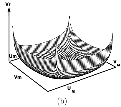
Fig. 4. (a) Image limits, (b) Repulsive potential for visibility
