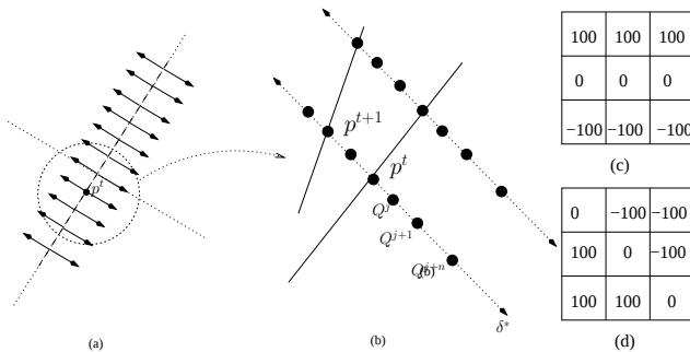
Fig. 2. Determining points position in the next image using the oriented gradient algorithm: (a) calculating the normal at sample points, (b) sampling along the normal (c-d) 2 out of 180 3x3 predetermined masks (in practice 7x7 masks are used) (c) 180° (d) 45°.
