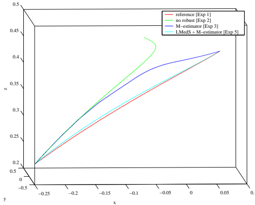
Fig. 5. Camera trajectory for important matching errors.
