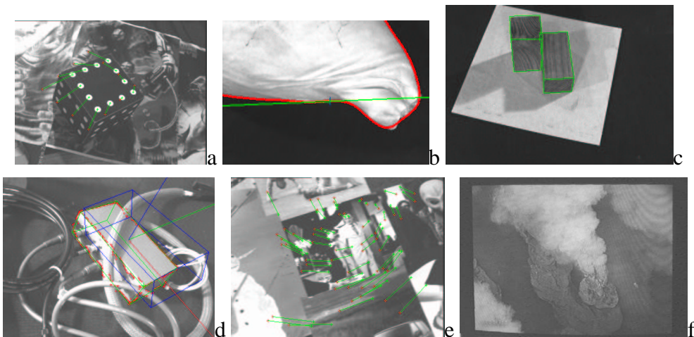
Figure 1. Features tracking in visual servoing experiments (ordered by subjective increasing difficulties) (a) tracking fiducial markers (b) tracking contours (c) 3D model-based tracking within “clean” environment (d) 3D model-based tracking in cluttered environment (e) tracking points of interest (f) tracking using motion estimation.
