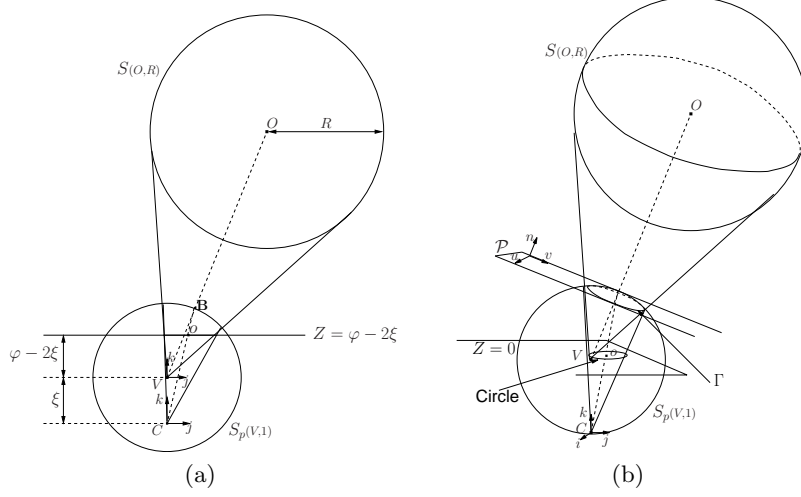
Fig. 2. Central catadioptric image of a sphere: (a) general case; (b) paracatadioptric projection ( \xi = 1 )
