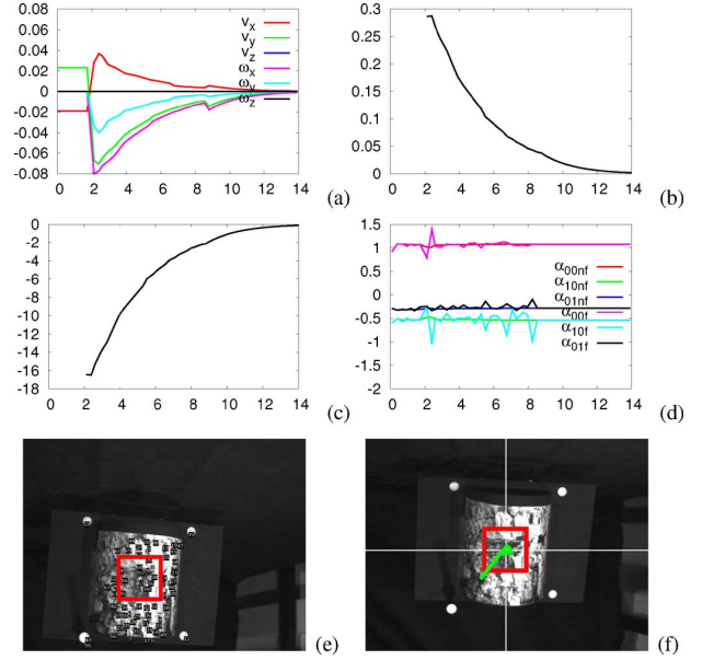
Fig. 9. Third experiment. Active vision. Cylinder. {}^d\Phi = (15^\circ, 0^\circ) .
