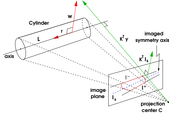
Fig. 1.7 A cylinder and its image with the perspective projection P . The backprojection of the apparent lines (I^-, I^+) is a pair of planes P^- I^- and P^+ I^+ , passing through the projection center. The image of the cylinder axis \Delta is the axis I_s of the harmonic homology H relating the apparent lines.
