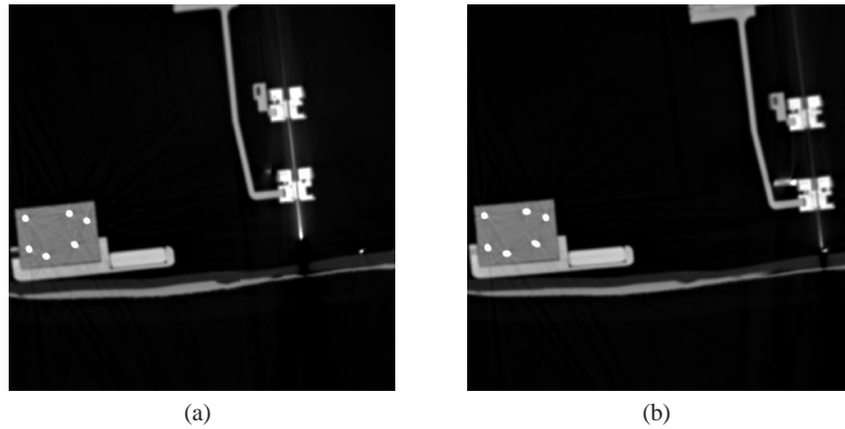
Fig. 1.8 "Look and move" with CT scanners. (a) The needle is maintained in the needle-holder jaws of a lightweight parallel robotic platform (CT-Bot), which has to be moved to the target point (right). (b) A new acquisition to check for the final positioning.
