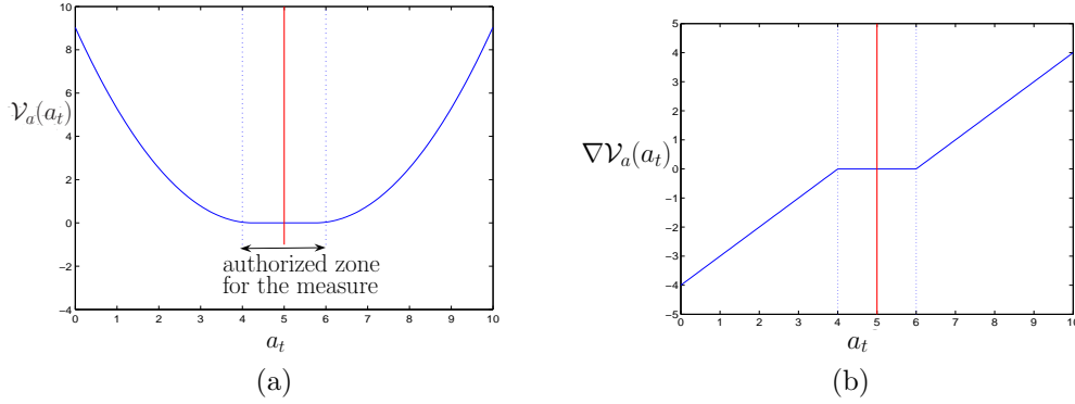
Figure 7: Controlling the motion along the optical axis: (a) the function used, (b) its gradient
