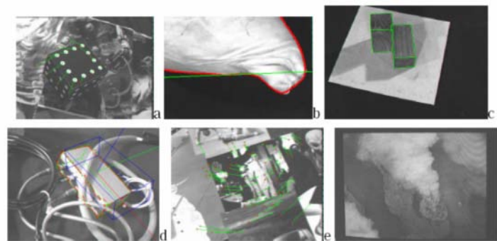
Figure 4: Features tracking in visual servoing experiments (ordered by subjective increasing difficulties) (a) tracking fiducial markers (b) tracking contours (c) 3D model-based tracking within “clean” environment (d) 3D model-based tracking in cluttered environment (e) tracking points of interest (f) tracking using motion estimation.
