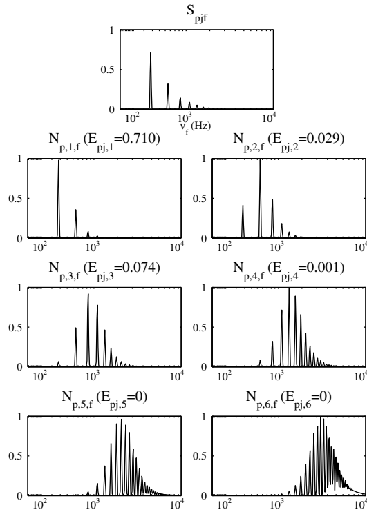
Figure 4: Basis spectrum S_{pj^f} estimated for the piano excerpt in Fig. 1 given fixed harmonic fine structure spectra N_{pk^f} ( p = 60 , gammatone windows of order n = 4 , b = 11/3 ERB, K_{\max} = 6 ).
