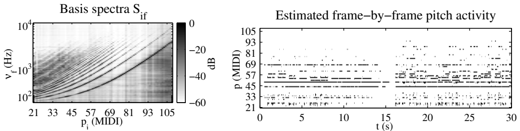
Figure 3: Basis spectra learned from the University of Iowa’s piano samples and resulting pitch activity derived for the piano excerpt in Fig. 1 via NMF.
