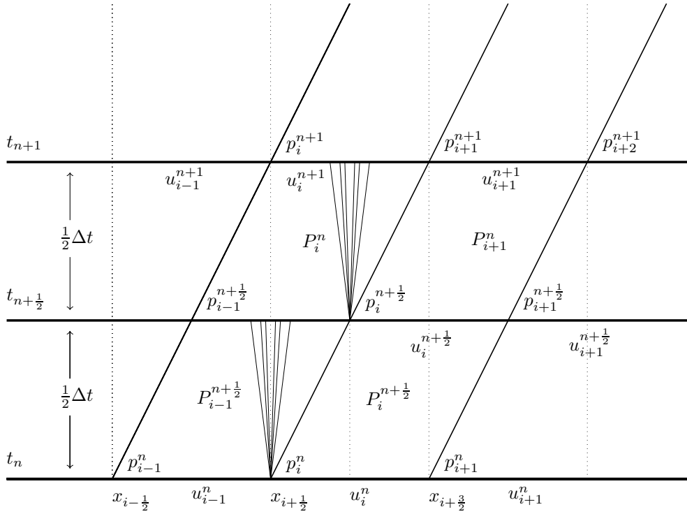
Figure 3.1: Notation for the two step monotонization scheme.
