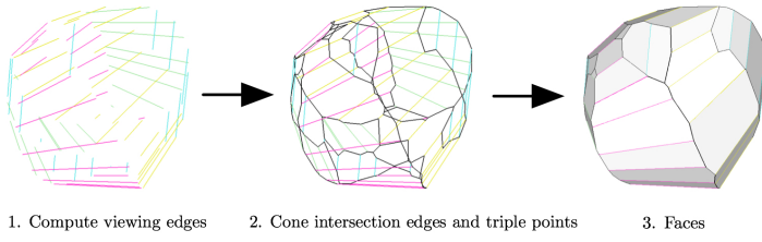
Fig. 5. Algorithm overview.
