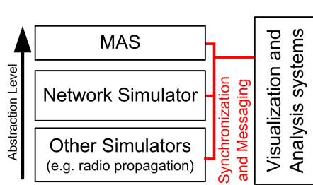
Fig. 5. Framework design
