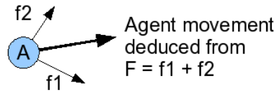
Fig. 4. Movement computation
