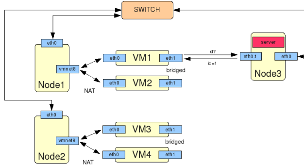
Figure 2: Network configuration
