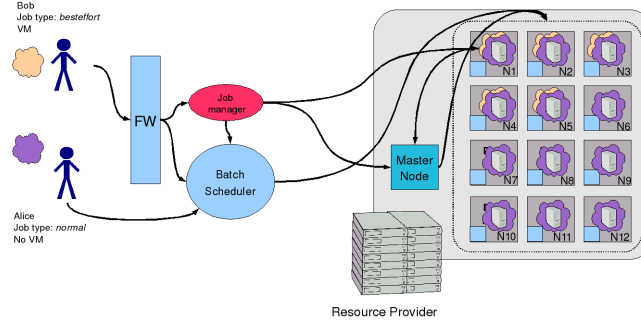
Figure 4: Architecture Overview
