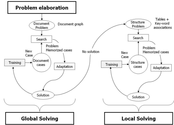
Figure 3. CBRDIA flow
