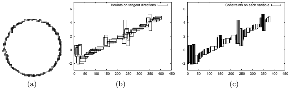
Fig. 5. Illustration of a distorted digital circle (a) with its tangent directions (b) and the constraints on each variable (c). The maximal blurred segments were obtained with width \nu = 3 .
