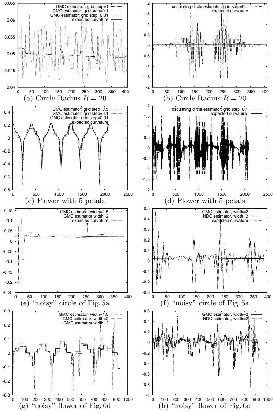
Fig. 7. Experimentations on regular (a-d) and damaged (e-h) contours. Plot (a) (resp. (c)) shows the curvature precision obtained on a quarter of circle R=20 (resp. flower) with several grid steps. Plots (b) and (d) show the results obtained by the osculating circle estimator. Curvature estimation precision on damaged shapes is shown on (e) and (g). A comparison between the GMC and NDC estimators is shown in (f,h).
